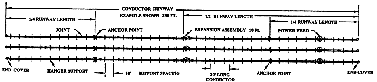
SCHEMATIC DIAGRAM
